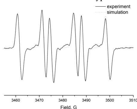
Fig.1. EPR experimental and simulated spectra of DMPO radical adduct following benzene adsorption on Cu/HZSM-5 in cyclohexane.
