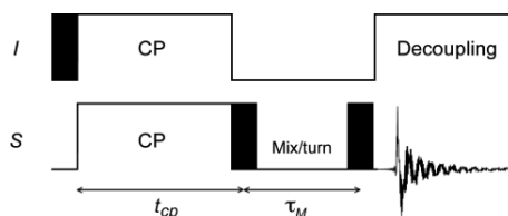
The RODEO-CP pulse sequence
