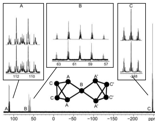
Figure 1 ^{31}\text{P} spectrum (161.99 MHz) of [\text{P}_9][\text{Al}(\text{OC}(\text{CF}_3)_3)_4] in \text{CH}_2\text{Cl}_2/\text{CD}_2\text{Cl}_2 at 298K (20000 scans, standard: aqua. \text{H}_3\text{PO}_4 (85%)). In the lower trace the experimental spectrum is shown. The boxes enlarge the individual signals of [\text{P}_9]^+ (lower trace: experimental spectrum, upper trace: calculated spectrum).
