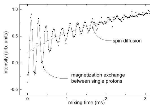
Fig.: Local proton magnetization exchange pattern observed in a host-guest liquid crystal
