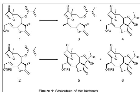
Figure 1: Structure of the lactones.
