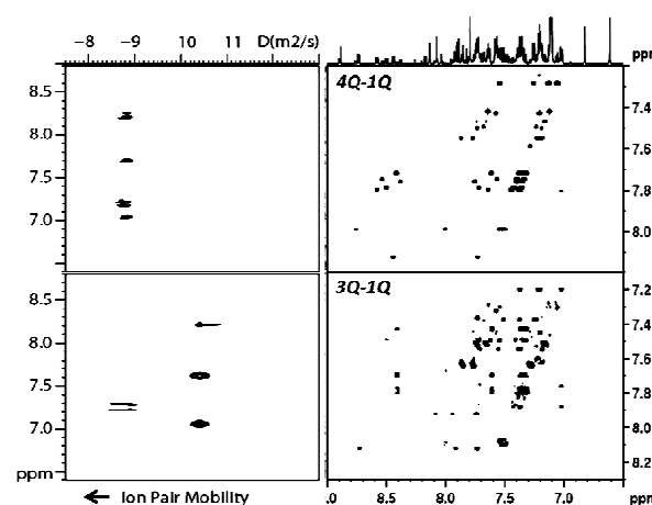
Chromatographic NMR on Fe 2+ pairs (left), MaxQ on 16 PAHs (right).
