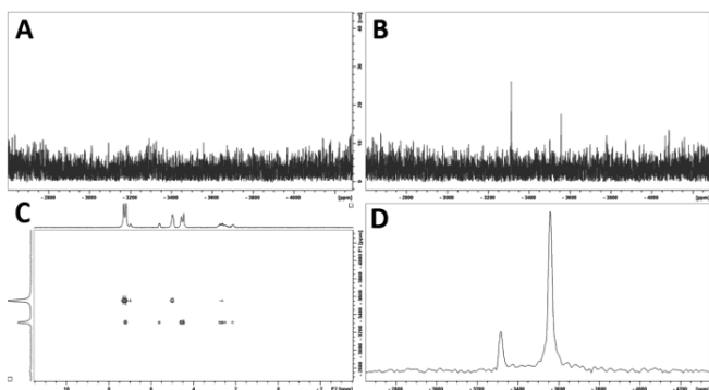
Figure 1: Example spectra for (COD)PtCl 2 with impurities; A: 1D-spectrum, 256 scans, 9 min 32 sec acquisition time, S/N = 1.86; B: 1D-spectrum, 1024 scans, 37 min 52 sec acquisition time, S/N = 7.13; C: ^1\text{H} , ^{195}\text{Pt} -HMBC, 2 scans, 128 increments, 10 min 38 sec acquisition time, S/N = 102.05; D: slice of the 2D-spectrum at 7.20 ppm.
