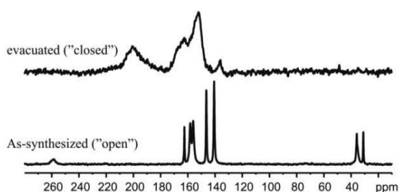
Fig. 1 ^{13}\text{C} CP MAS NMR spectra of DUT-8 (Ni)
