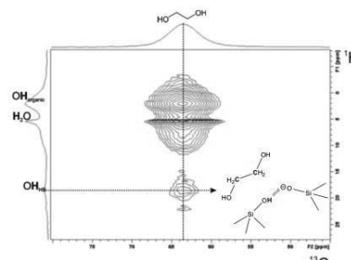
Figure. 1 H- 13 C HETCOR NMR spectra of a silica/ethylene glycol hydrogel.
