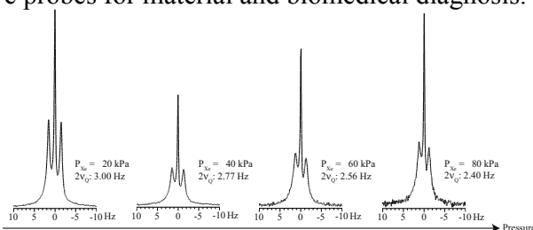
Fig. 1. NMR spectra of hp ^{131}\text{Xe} at different pressures on a glass surface. The quadrupolar splitting of the ^{131}\text{Xe} decreases as the pressure of xenon gas increase. This decrease is attributed to changes in the gas phase contribution of the 2\nu_Q given that the surface is unchanging between experiments.
