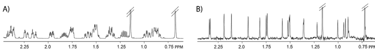
Figure 1; A) 1D proton NMR spectrum of testosterone B) Spectrum of 500μM testosterone free from homonuclear J-couplings
