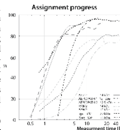
Fig. 1. Progress of the automated assignment for several protein systems. Slope of the curves is defined mainly by the S/N in the spectra. Level of the final plateau depends on the spectra intensity range and presence of weak or missing spin systems
