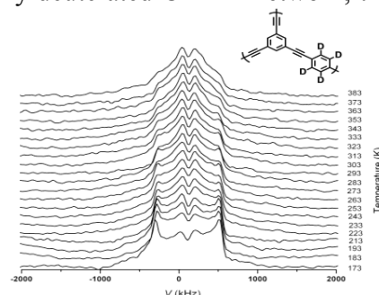
Figure: 2 H VT NMR and structure (inset) of deuterated CMP-1.
